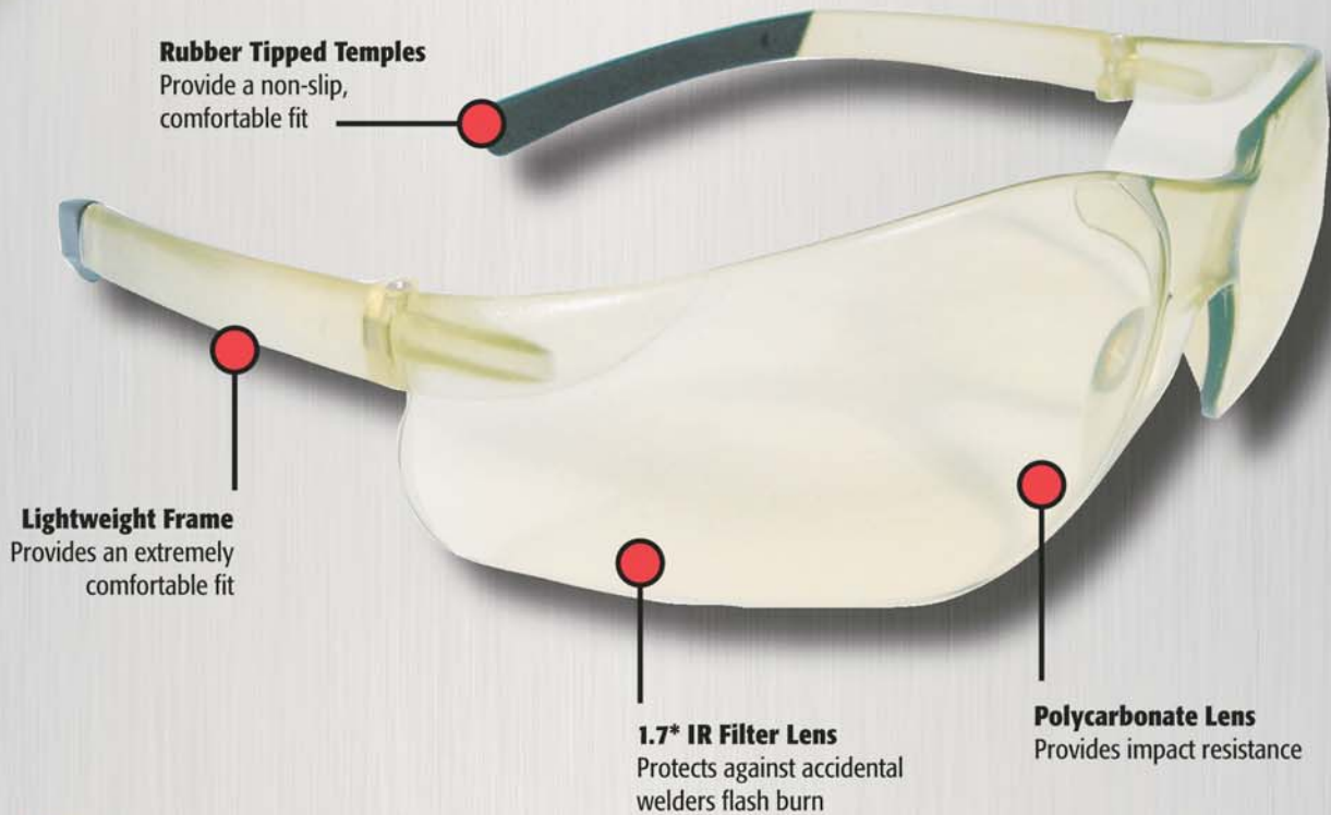
AT1-W2 1.7* IR Filter Lens
